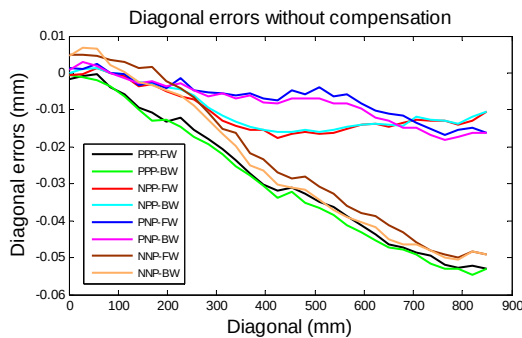
Fig. 13: Diagonal error without compensation
