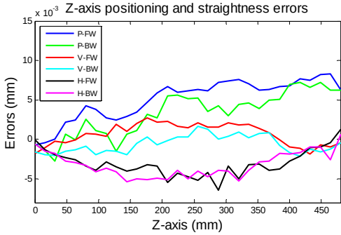
Fig. 16: Z-axis errors with compensation
