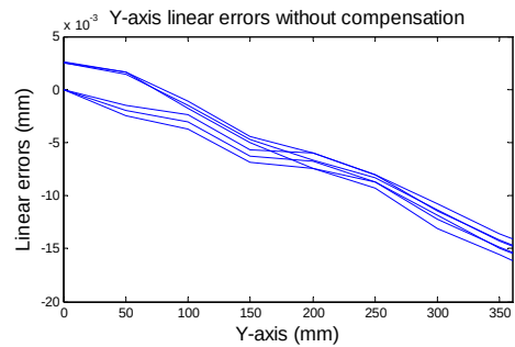
Fig. 8: Y-axis linear positioning errors
