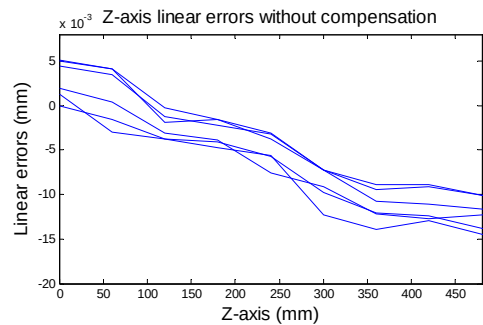
Fig. 9: Z-axis linear positioning errors
