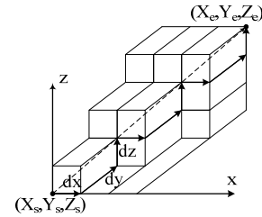
Fig. 5: Principle of vector step diagonal measurement
