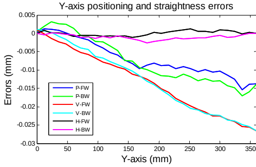
Fig. 11: Y-axis errors without compensation
