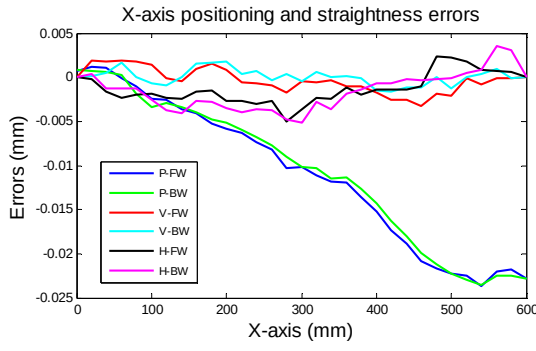
Fig. 10: X-axis errors without compensation
