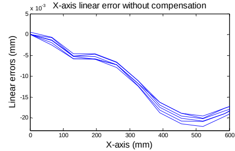
Fig. 7: X-axis linear positioning errors
