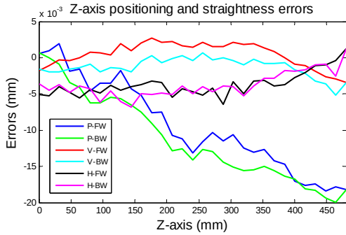
Fig. 12: Z-axis errors without compensation
