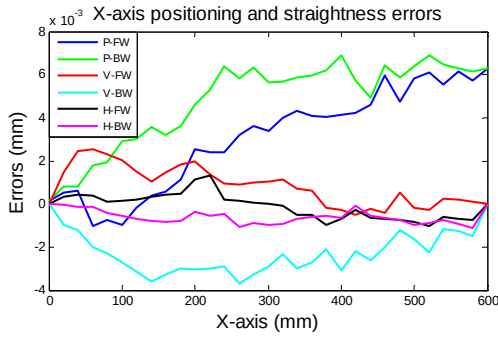
Fig. 14: X-axis errors with compensation
