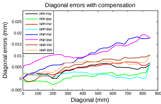
Fig. 17: Diagonal errors with compensation
