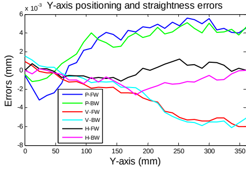
Fig. 15: Y-axis errors with compensation
